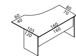
Y-40 160-40/105-70/75
