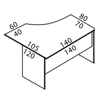
Y-36 140-40/105-70/75
